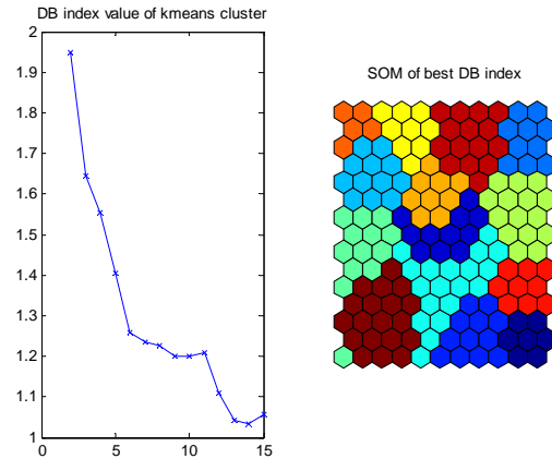
Fig. 11 Davies-Boulding clustering index (left figure), and SOM cluster by color code which is minimized with best clustering (right figure). Training data are 1205 texts of 500 concept features.
